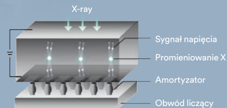
Czujnik Xpect Vision
